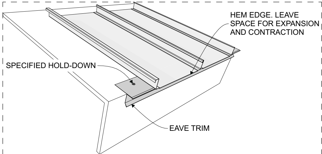
A | EAVE TRIM
