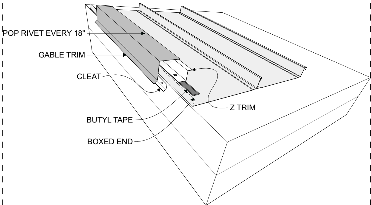
C | GABLE TRIM
