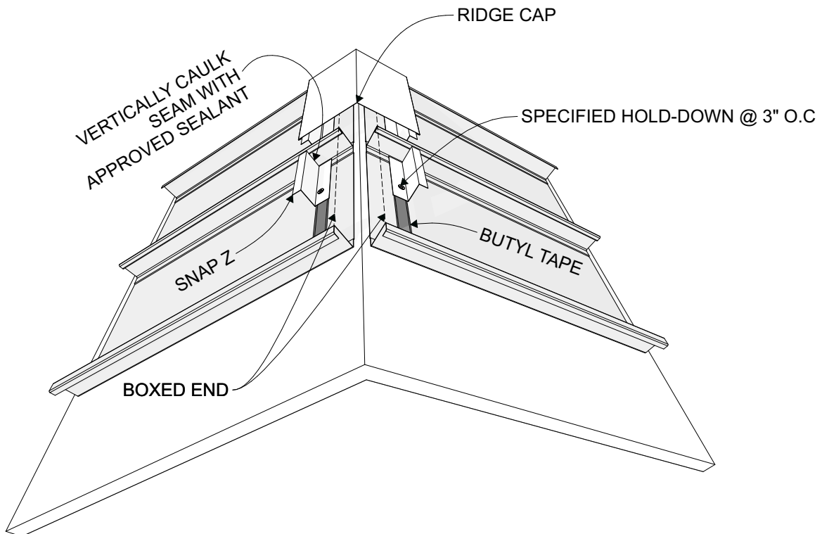
G | RIDGE CAP
