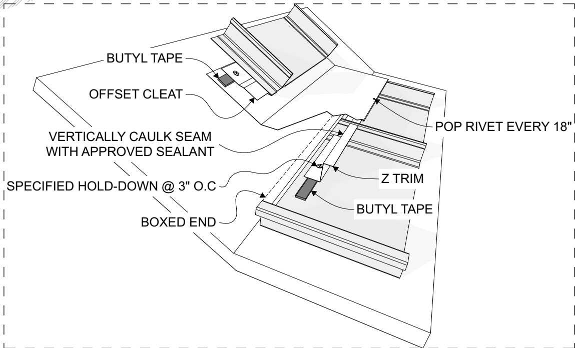
F | PITCH BREAK
