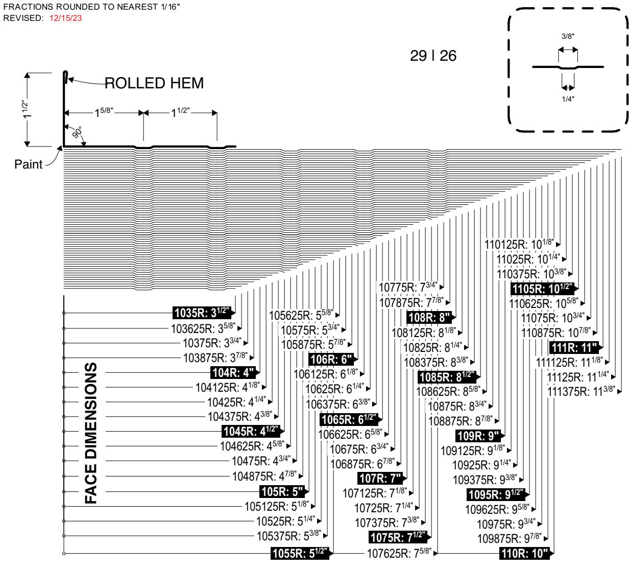
A1 Profile Section Detail Scale: 6" = 1'-0"
